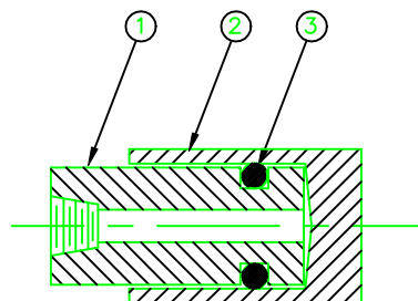
HEAD STEAM CYLINDER(No.11) (PART No.A-4240)
